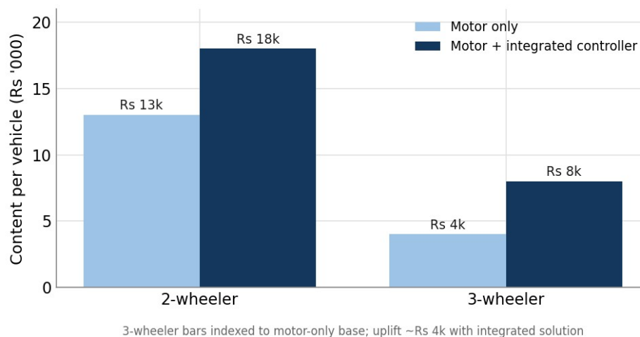
EXHIBIT 4: 2W/3W content per vehicle: motor-only versus integrated (Rs '000)
